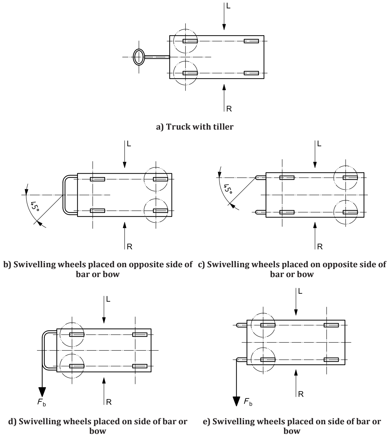
Figure A.4 — Position of the wheels and direction of the force at the beginning of measurement
