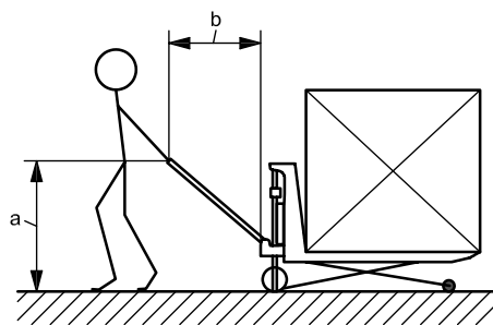
Figure 6 — Height of tiller handle
